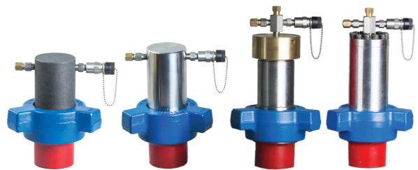
Sensor, Diaphragm Protector, Piston Isolator or Deboostor
