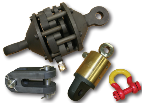
Clevis, Load Cell, Tension Cylinder and Shackle
