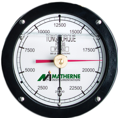
6" Power Tong Gauge Panel Mount
